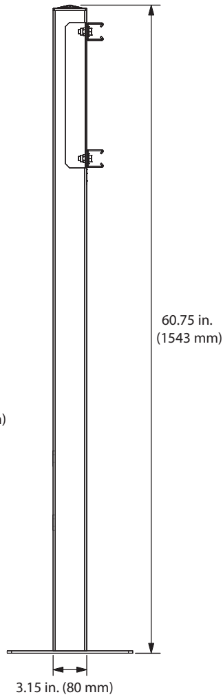
Side View
