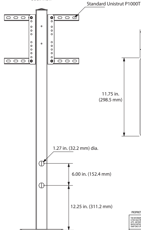
Back View
