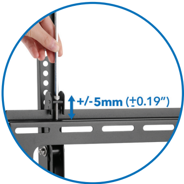
Screen leveling
